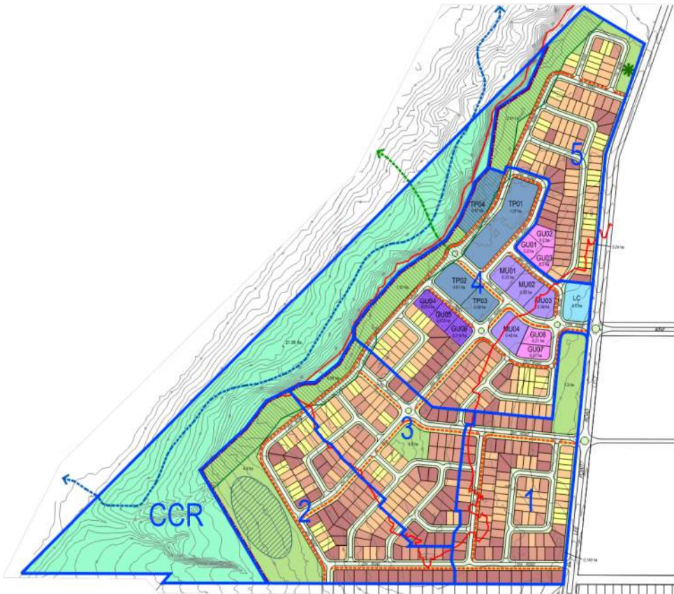
Figure 1-2 Proposed staging
